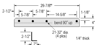
1. WAB13S00402 Brace
