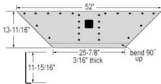
1. WAB13S00379 Jost
