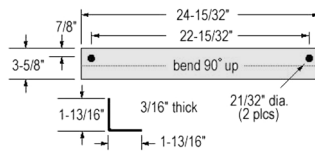
1. WAB13S00542 Brace
