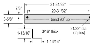
1. WAB13S00543 Brace
