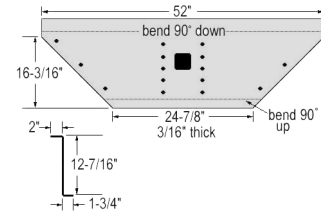
1. WAB13S00405 Jost
